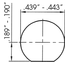
RECOMMENDED MOUNTING HOLE DIMENSIONS (inches)
