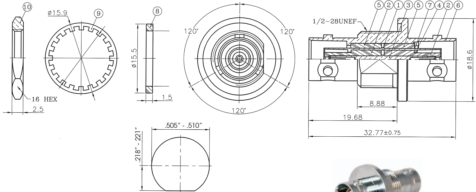
RECOMMENDED MOUNTING HOLE DIMENSIONS (inches)
